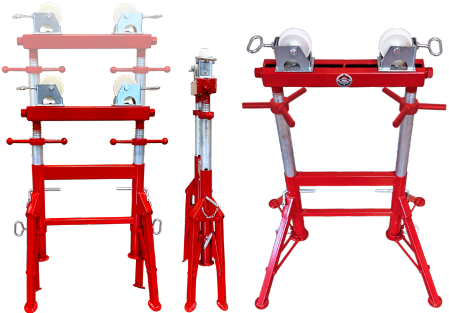
Folded Closed
